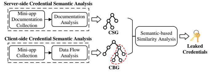
Fig. 2. KeyMagnet Workflow
